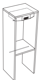
75x65x h210 cm colonna per smart dry column for smart dry
